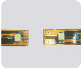
Step1:Two strips to be connected
