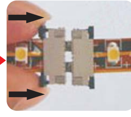
Step4: The same as step 3
