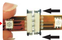
Step4: The same as step 3
