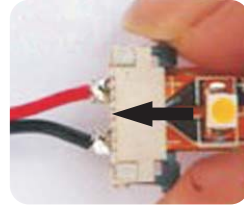
Step3 :Close the slot
